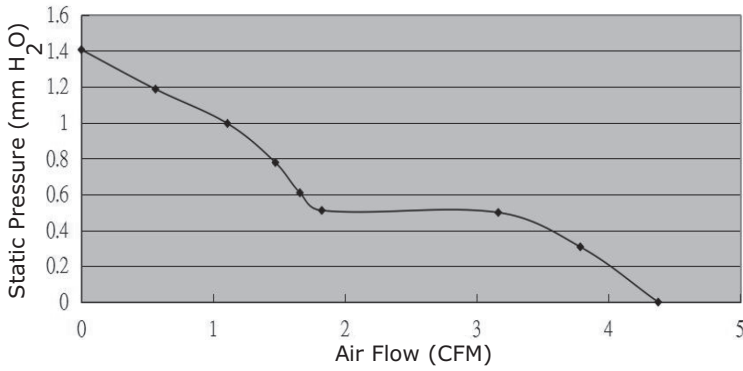
CFM-4020BF-035-114
