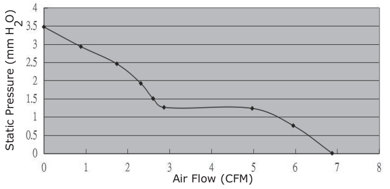
CFM-4020BF-055-212
